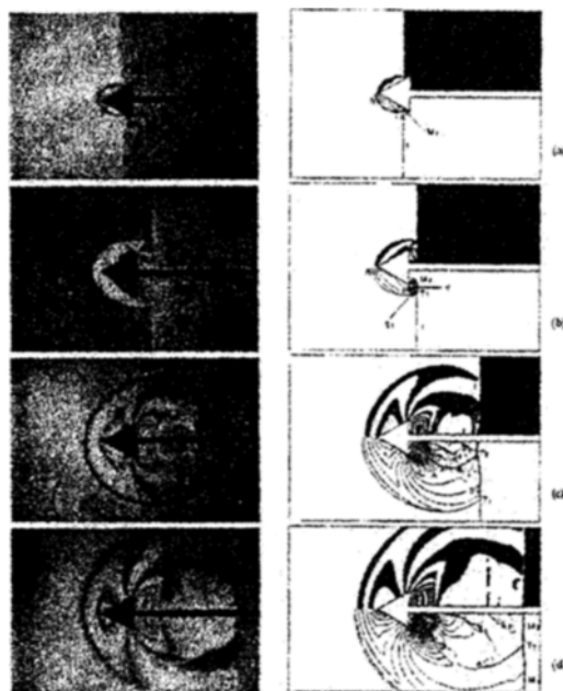
Fig. 4 Experimental interferogram (left), numerical isopycnics (lower right) and numerical interferogram (upper right), M_s=1.73 . (a) 24\mu s ; (b) 38\mu s ; (c) 98\mu s ; (d) 139\mu s
